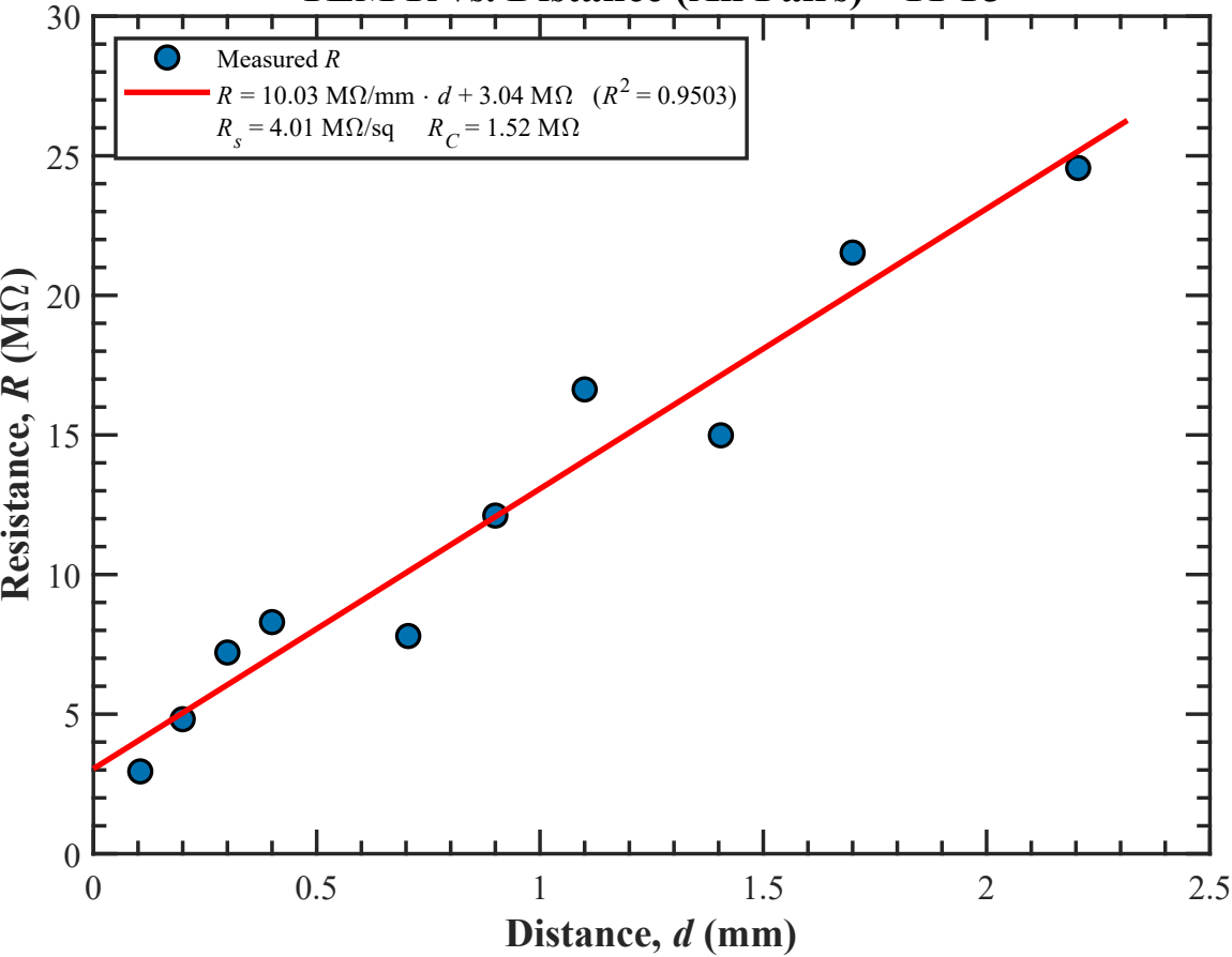
TLM R vs. Distance (All Pairs) - TFT3
